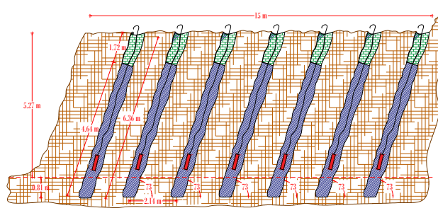
Right view 1:100
